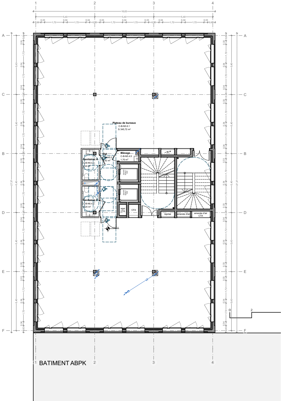
PLAN N5
