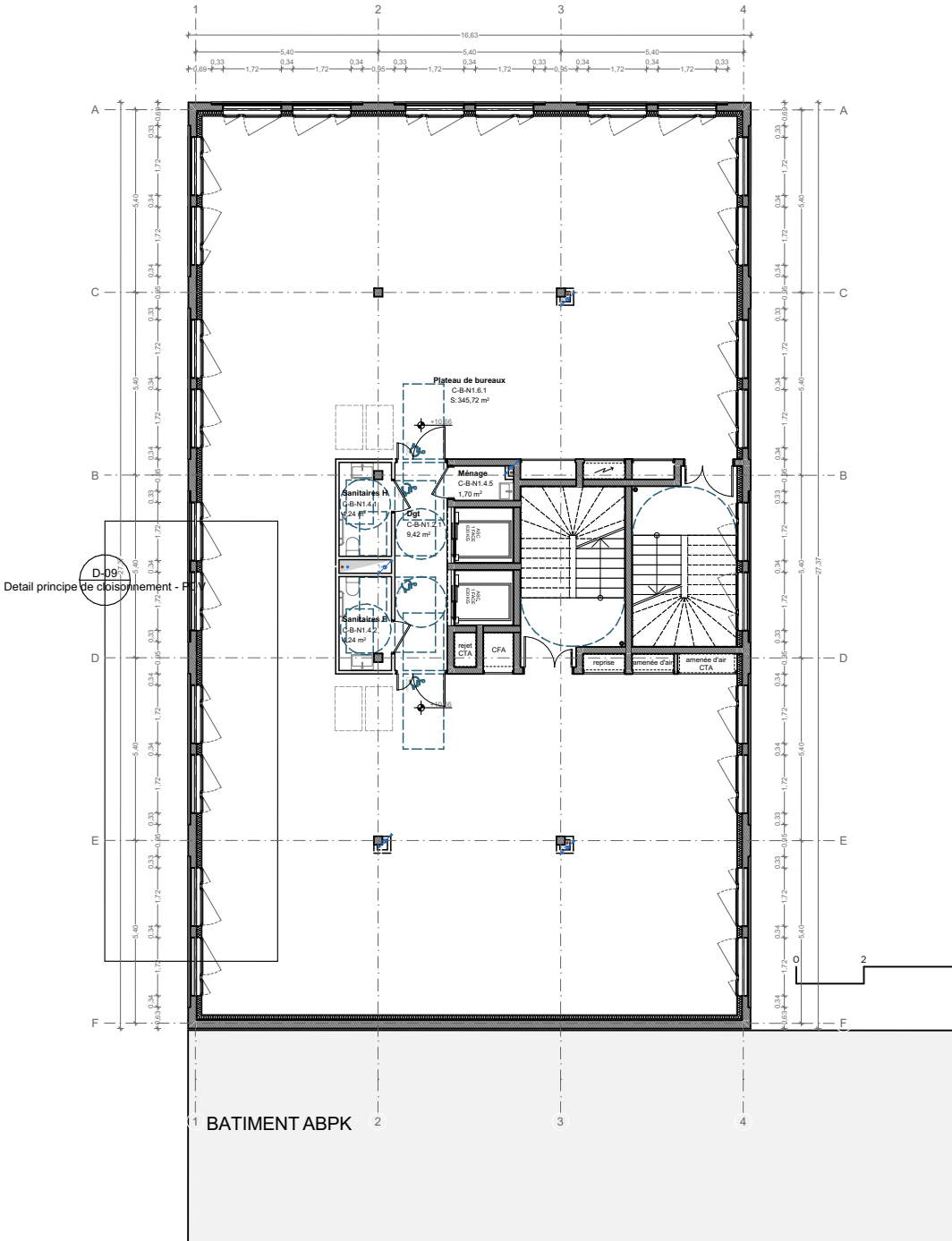
PLAN N1
