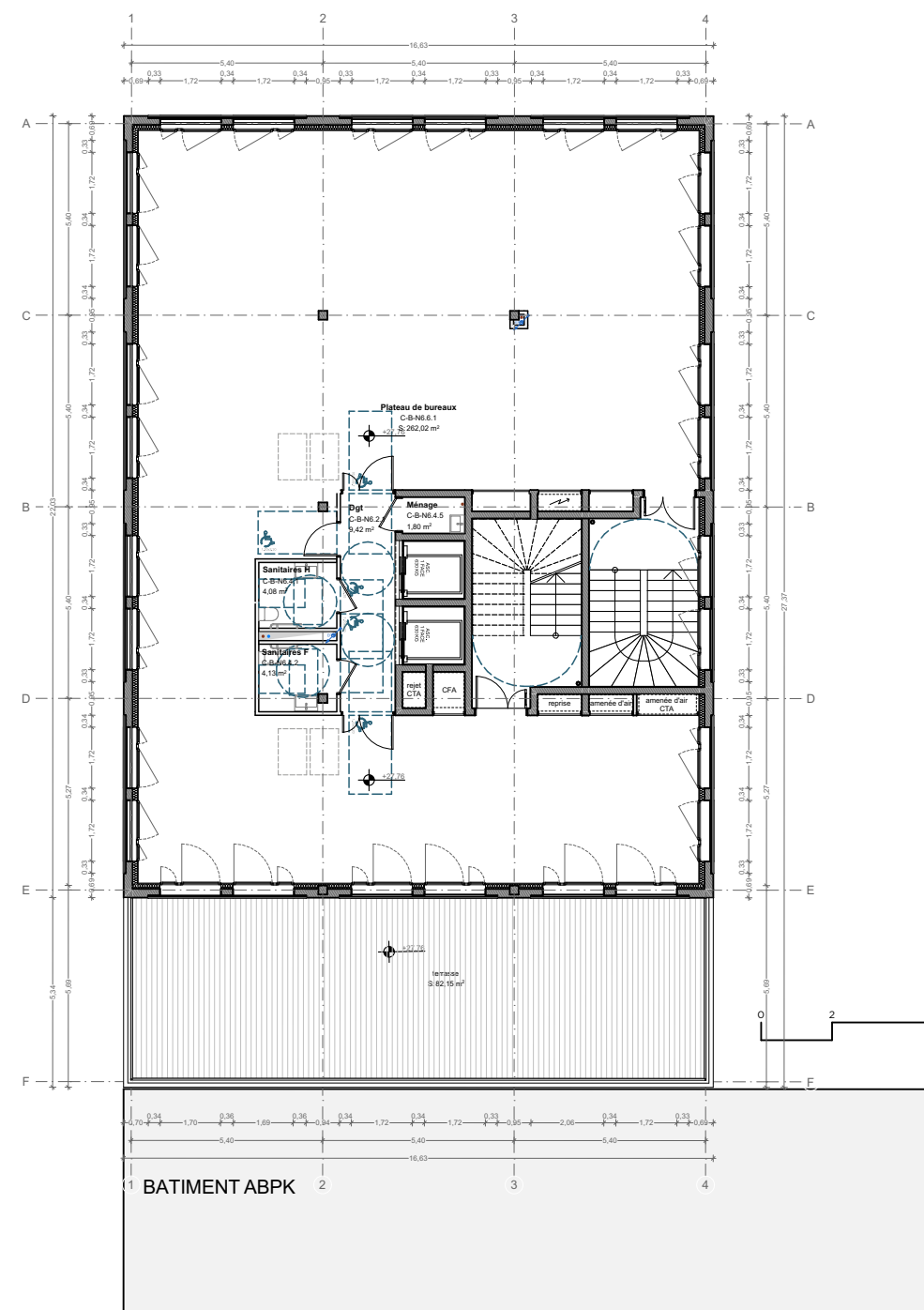
PLAN N6
