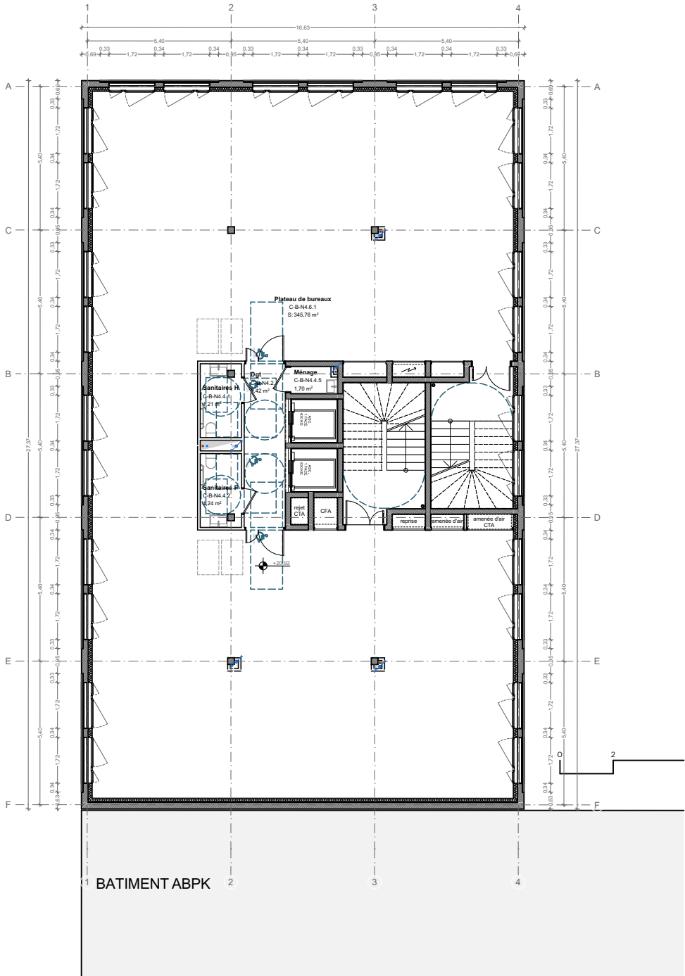
PLAN N4
