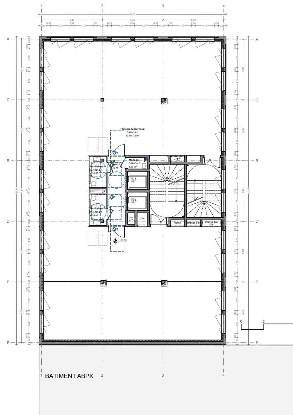
PLAN N3
